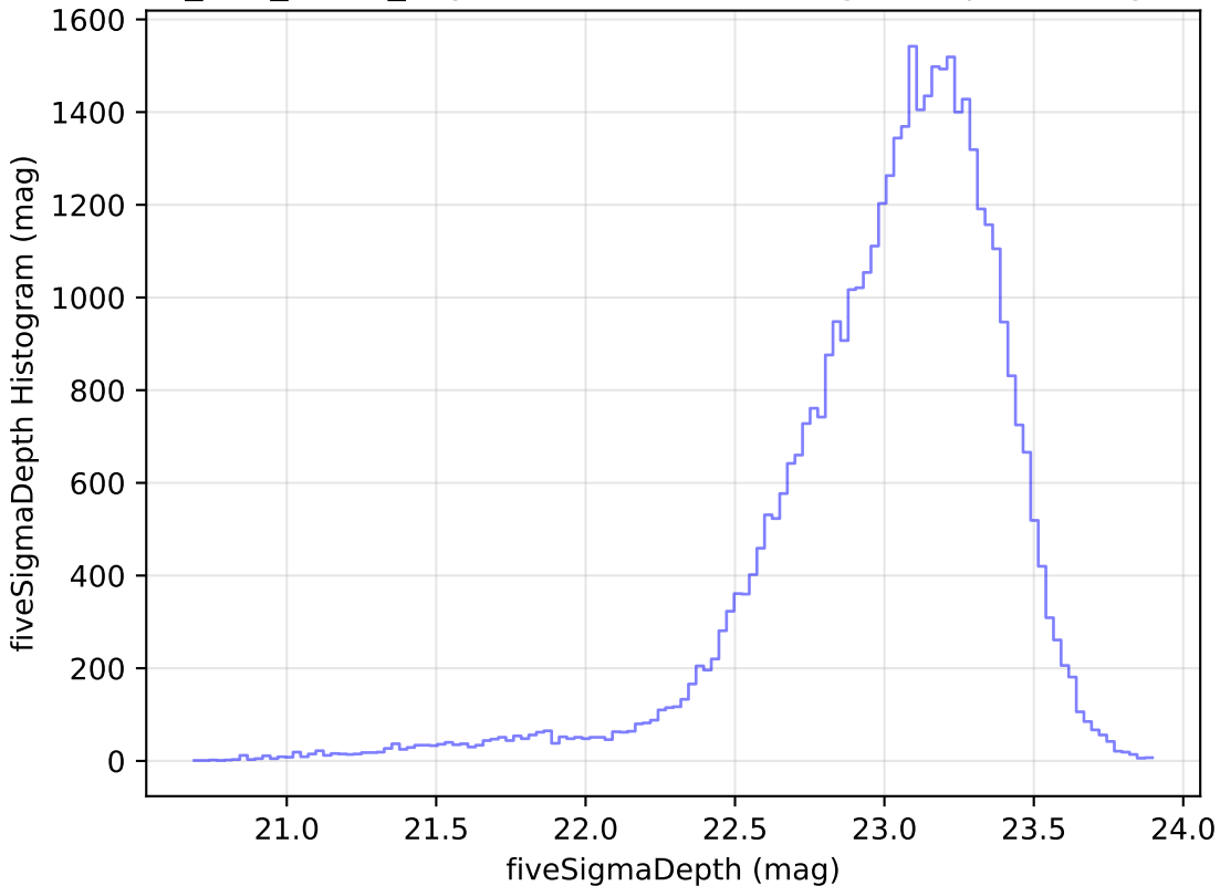
too_100_4v3.4_10yrs Yr 1 z band: fiveSigmaDepth Histogram
