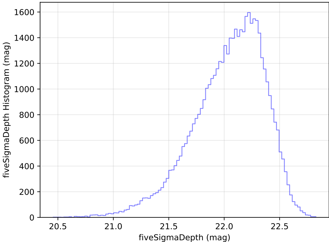
too_100_4v3.4_10yrs Yr 1 y band: fiveSigmaDepth Histogram
