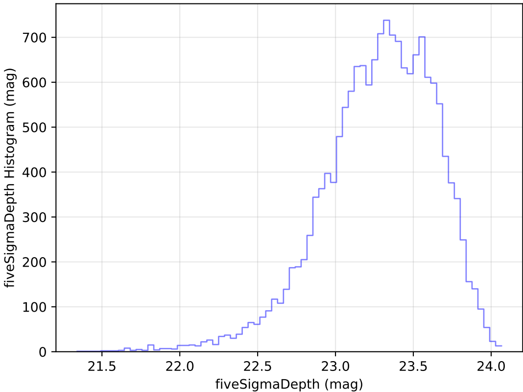
too_100_4v3.4_10yrs Yr 1 u band: fiveSigmaDepth Histogram
