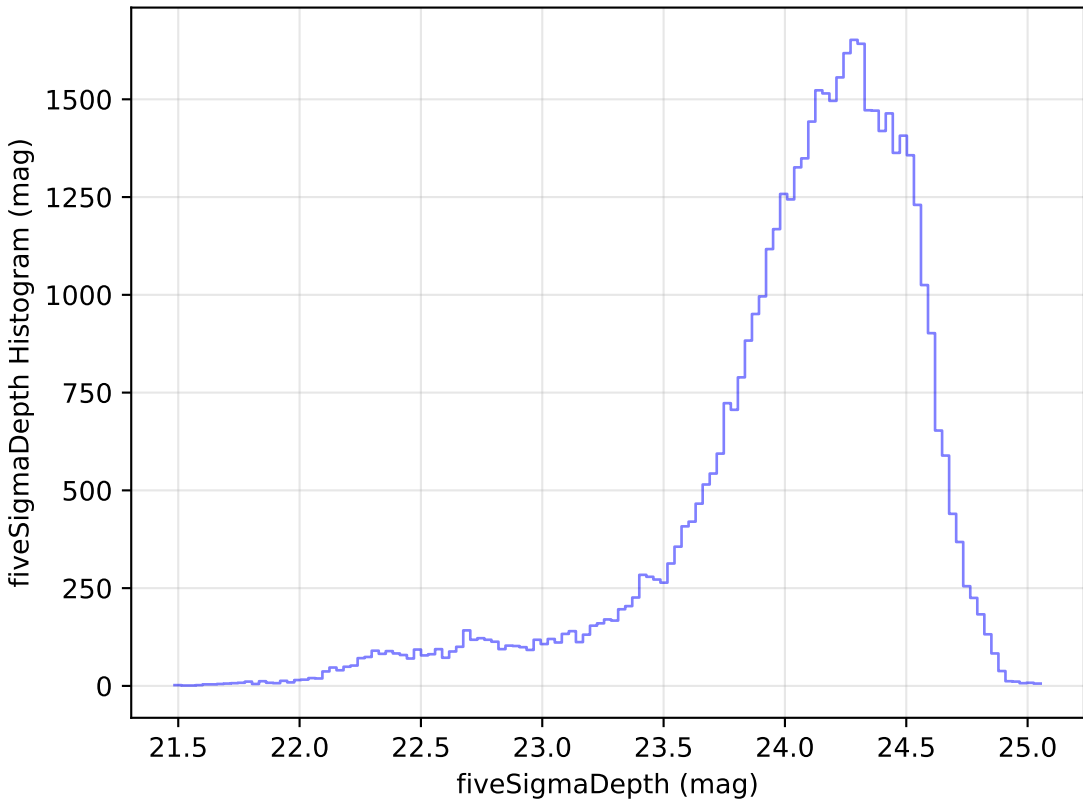
too_100_4v3.4_10yrs Yr 1 r band: fiveSigmaDepth Histogram
