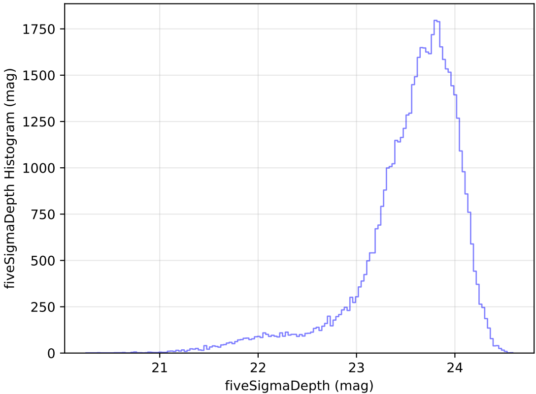
too_100_4v3.4_10yrs Yr 1 i band: fiveSigmaDepth Histogram
