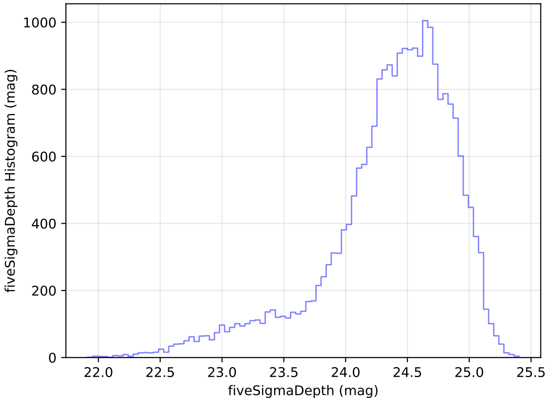
too_100_4v3.4_10yrs Yr 1 g band: fiveSigmaDepth Histogram
