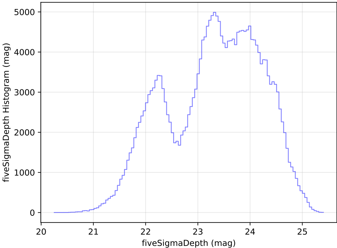
too_100_4v3.4_10yrs Yr 1 all bands: fiveSigmaDepth Histogram
