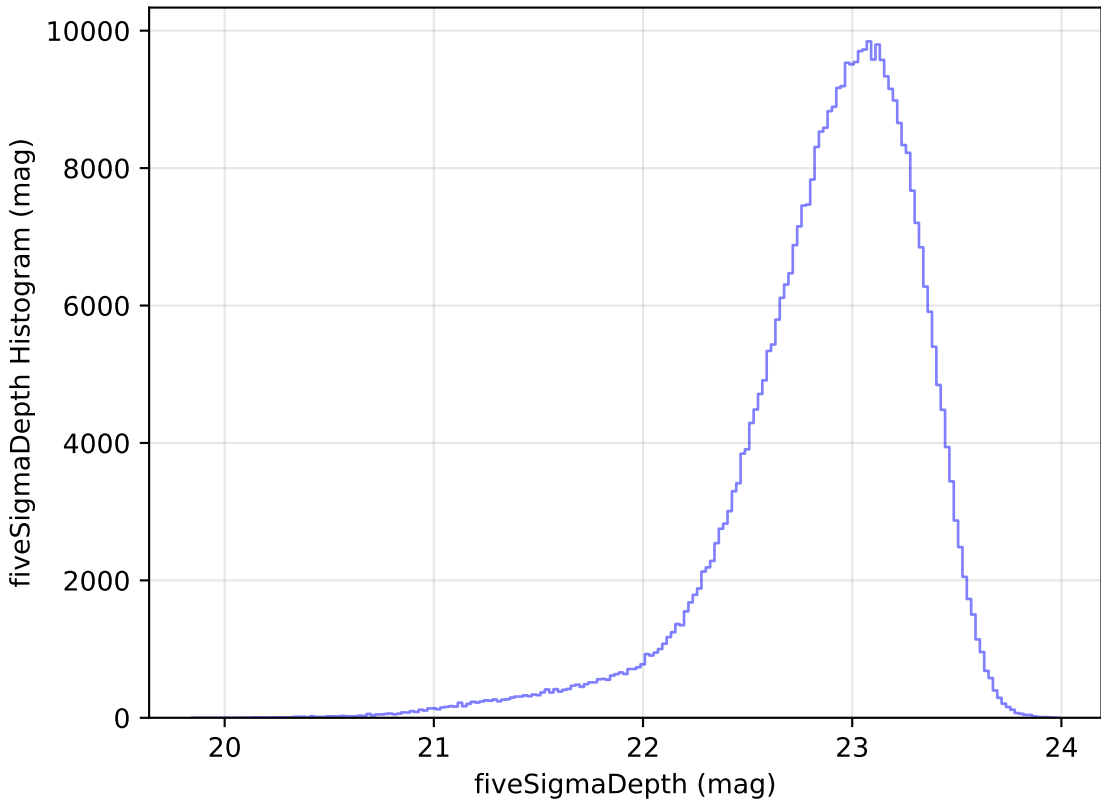
too_100_4v3.4_10yrs WFD z band: fiveSigmaDepth Histogram
