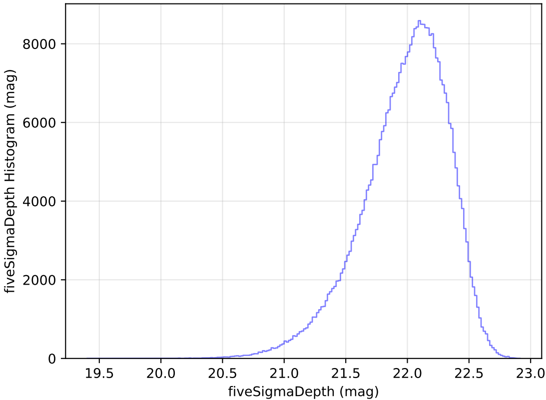
too_100_4v3.4_10yrs WFD y band: fiveSigmaDepth Histogram
