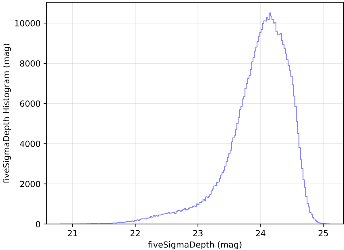
too_100_4v3.4_10yrs WFD r band: fiveSigmaDepth Histogram
