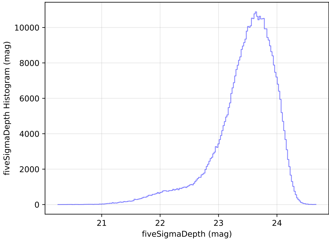
too_100_4v3.4_10yrs WFD i band: fiveSigmaDepth Histogram
