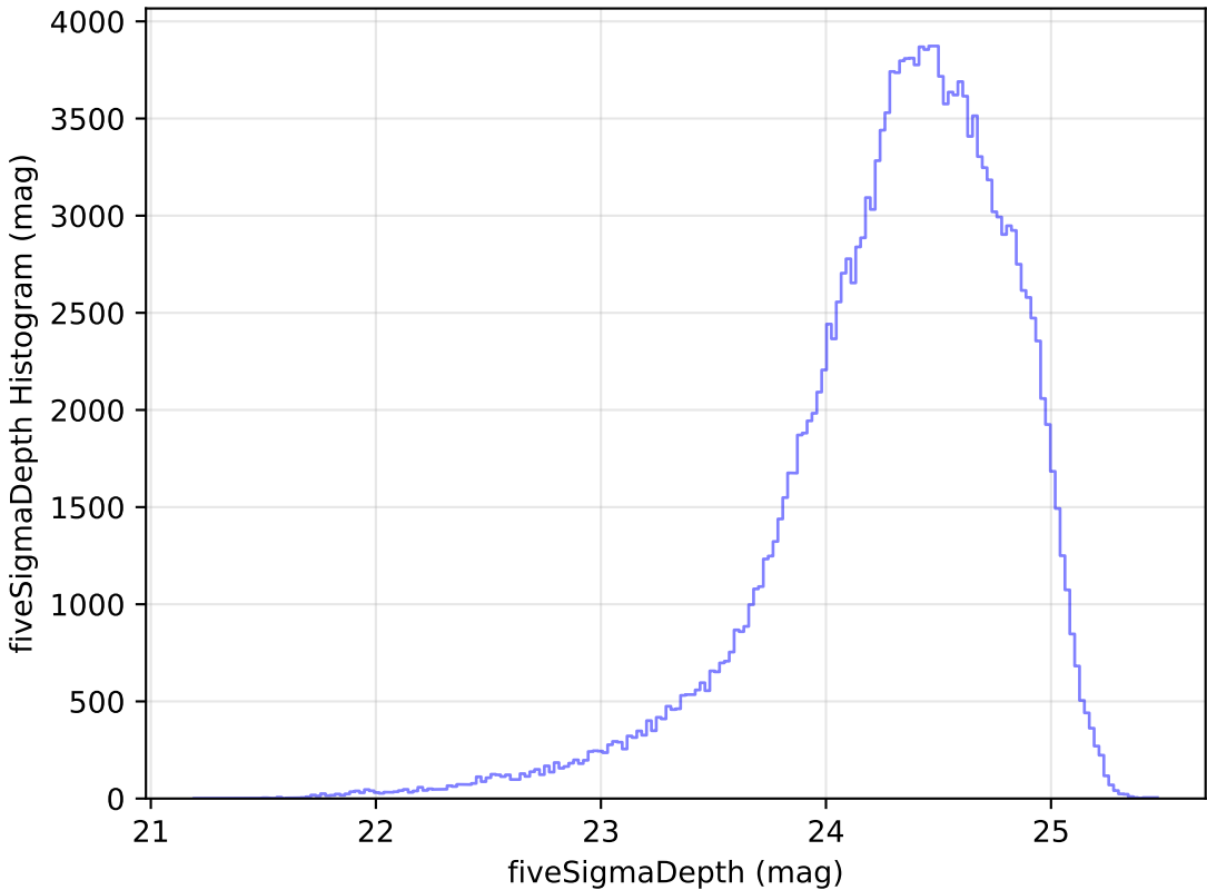
too_100_4v3.4_10yrs WFD g band: fiveSigmaDepth Histogram
