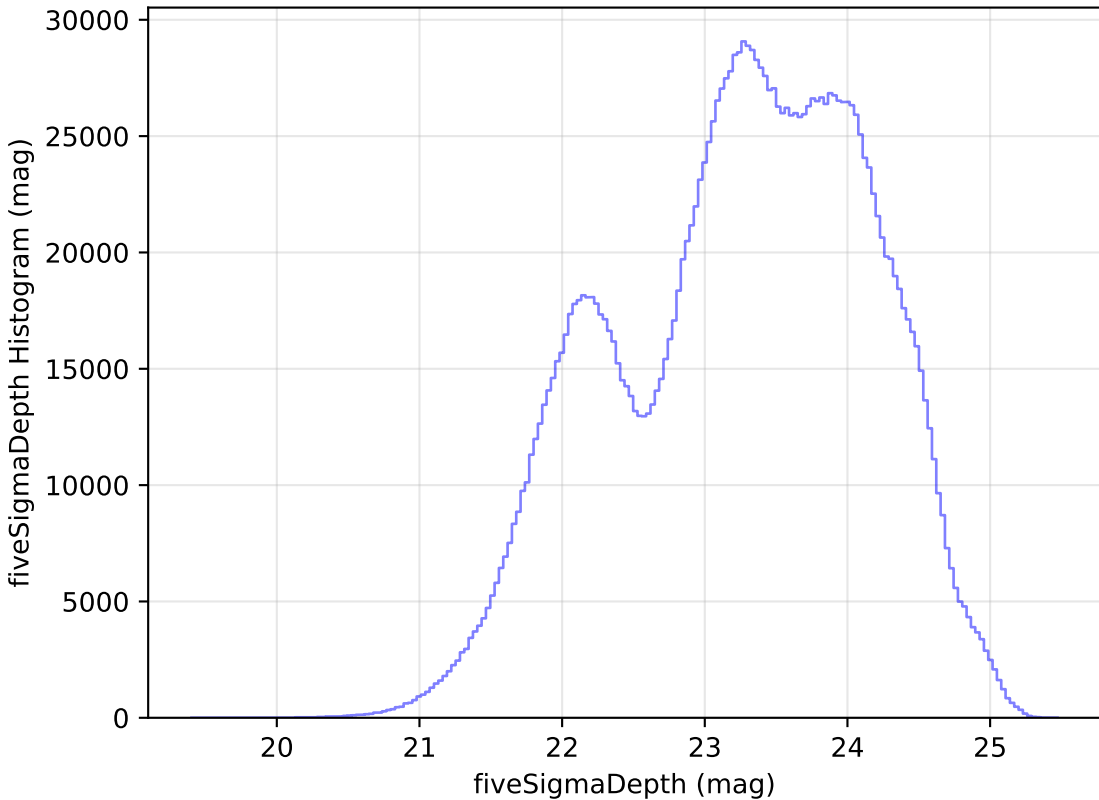
too_100_4v3.4_10yrs WFD all bands: fiveSigmaDepth Histogram
