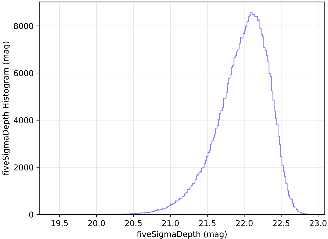
too_100_4v3.4_10yrs All sky y band: fiveSigmaDepth Histogram
