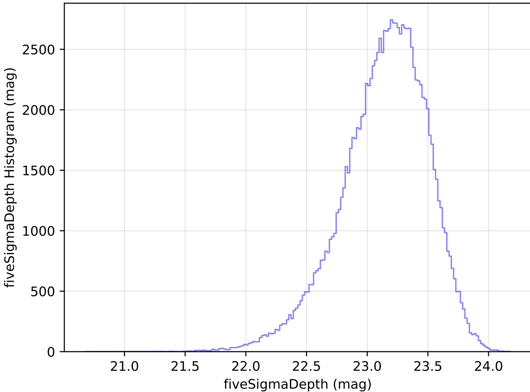
too_100_4v3.4_10yrs All sky u band: fiveSigmaDepth Histogram
