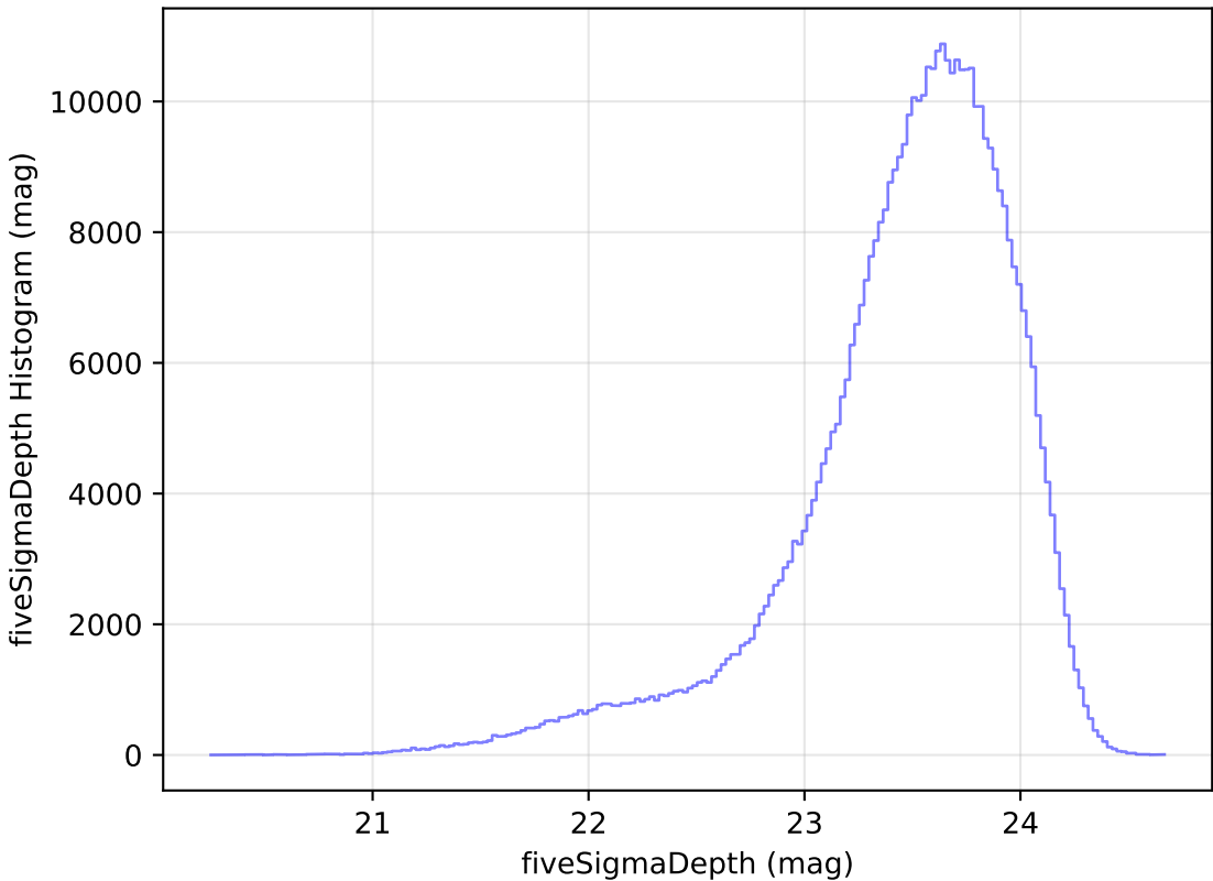
too_100_4v3.4_10yrs All sky i band: fiveSigmaDepth Histogram
