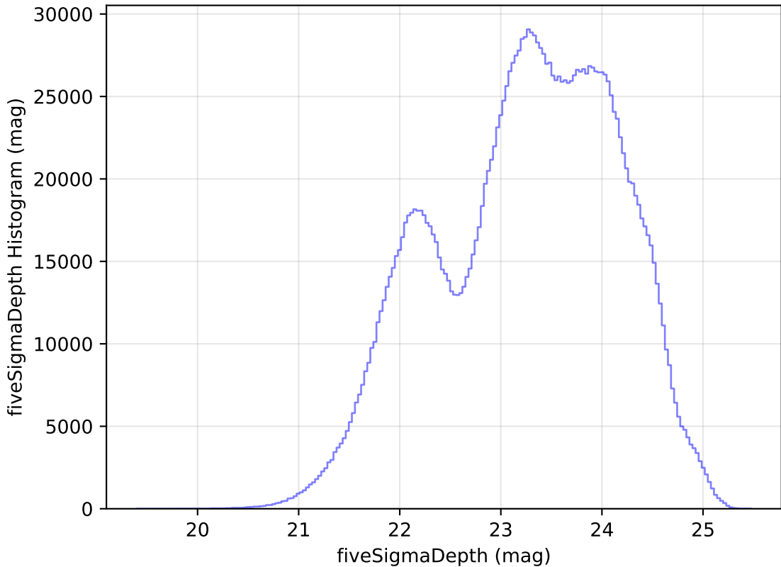
too_100_4v3.4_10yrs All sky all bands: fiveSigmaDepth Histogram
