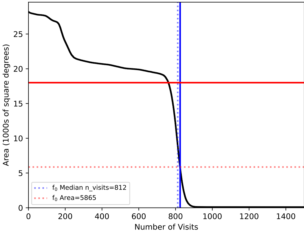
too_100_4v3.4_10yrs All sky: fO
