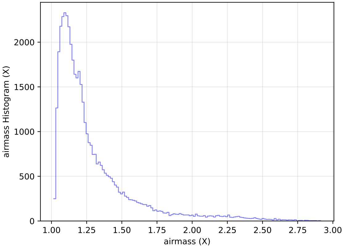
too_100_4v3.4_10yrs Yr 1 z band: airmass Histogram
