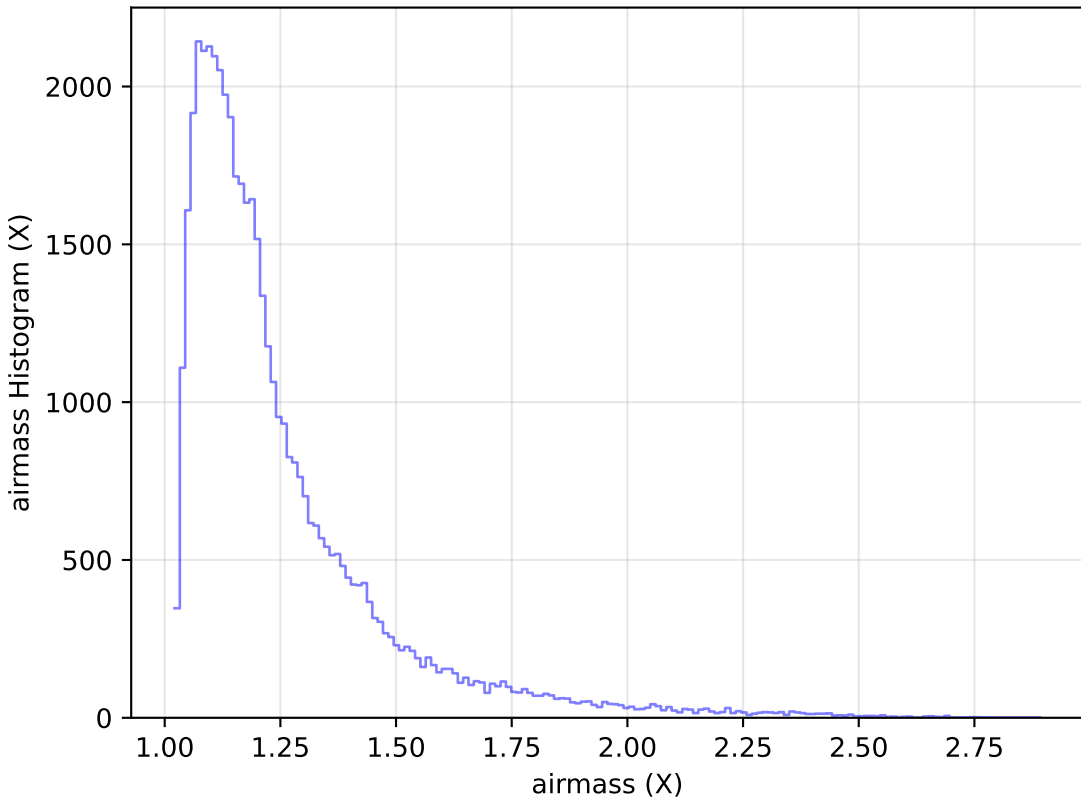
too_100_4v3.4_10yrs Yr 1 y band: airmass Histogram
