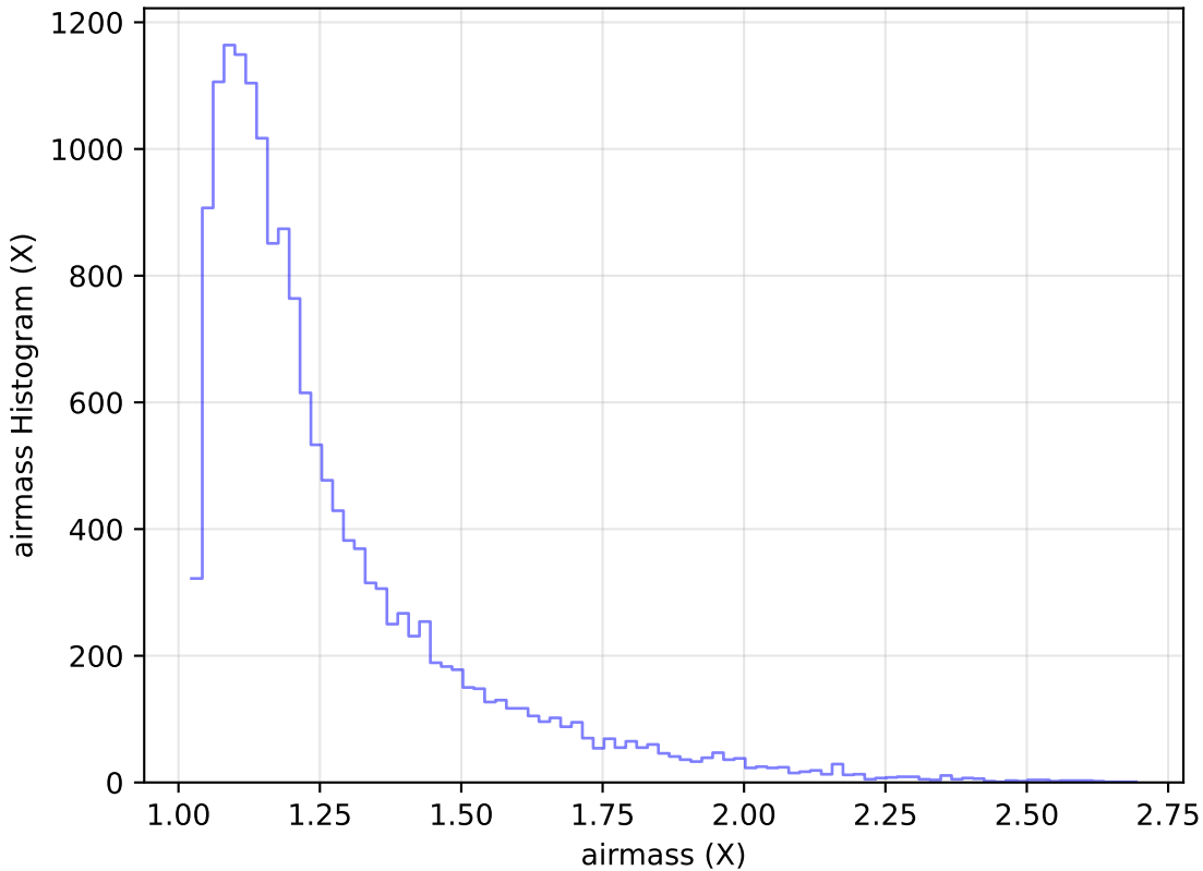
too_100_4v3.4_10yrs Yr 1 u band: airmass Histogram
