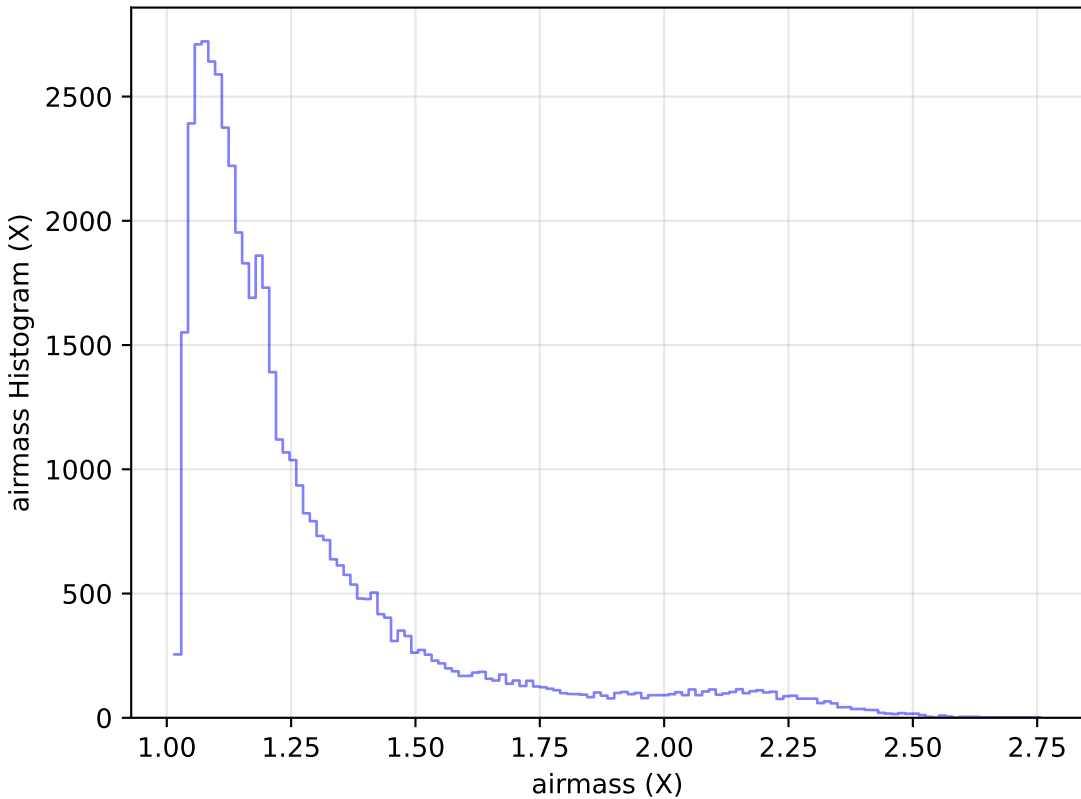
too_100_4v3.4_10yrs Yr 1 r band: airmass Histogram
