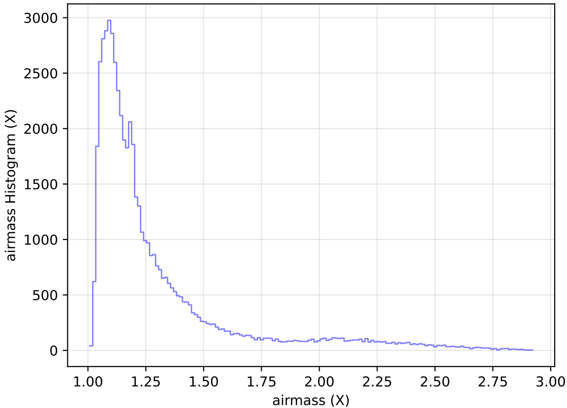
too_100_4v3.4_10yrs Yr 1 i band: airmass Histogram
