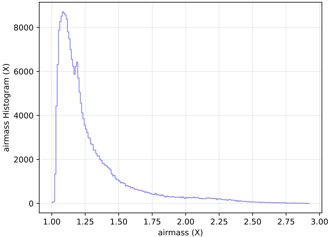
too_100_4v3.4_10yrs Yr 1 all bands: airmass Histogram
