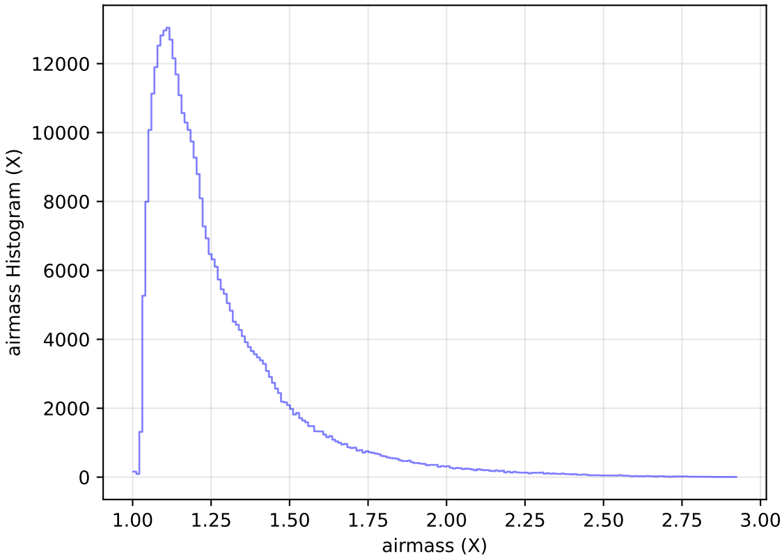
too_100_4v3.4_10yrs WFD y band: airmass Histogram
