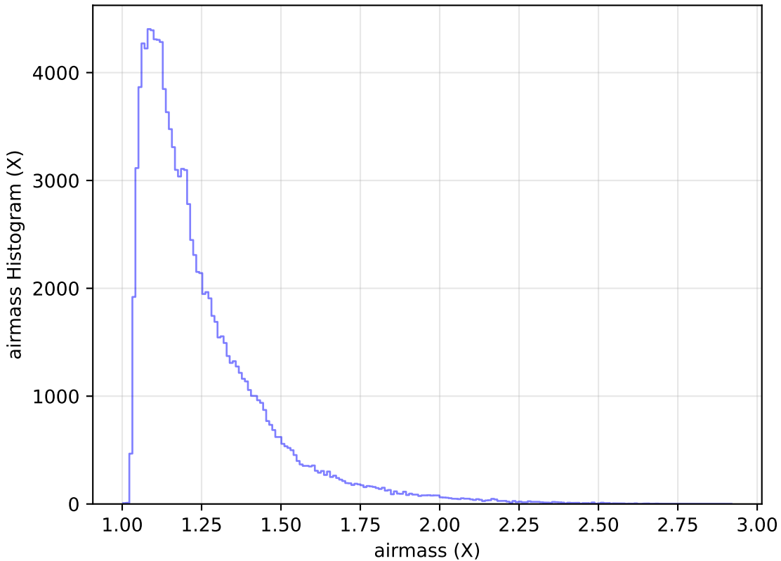
too_100_4v3.4_10yrs WFD u band: airmass Histogram
