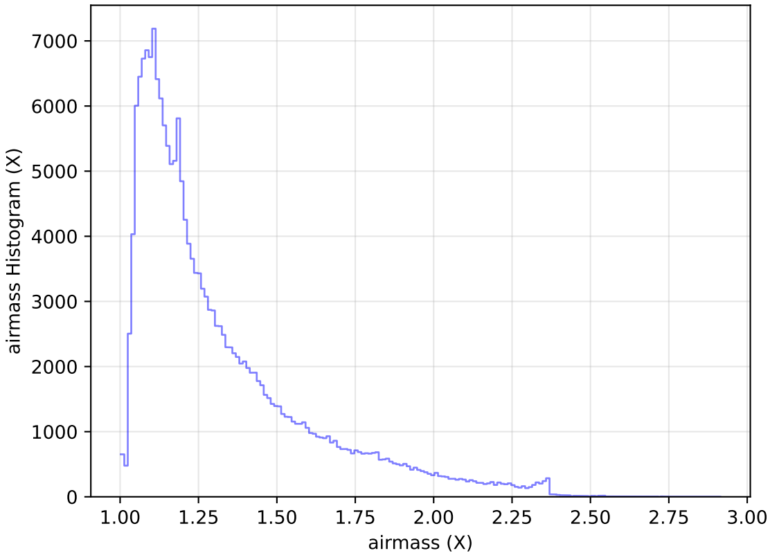
too_100_4v3.4_10yrs WFD g band: airmass Histogram
