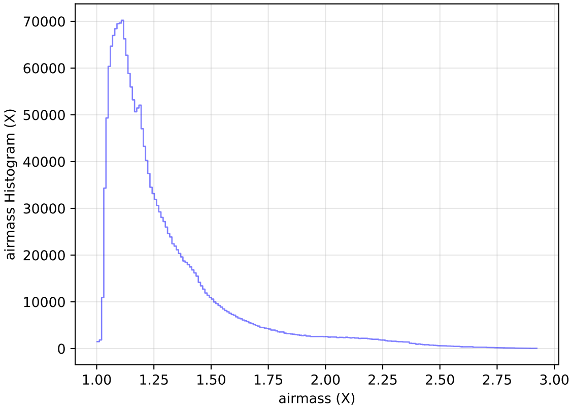
too_100_4v3.4_10yrs WFD all bands: airmass Histogram
