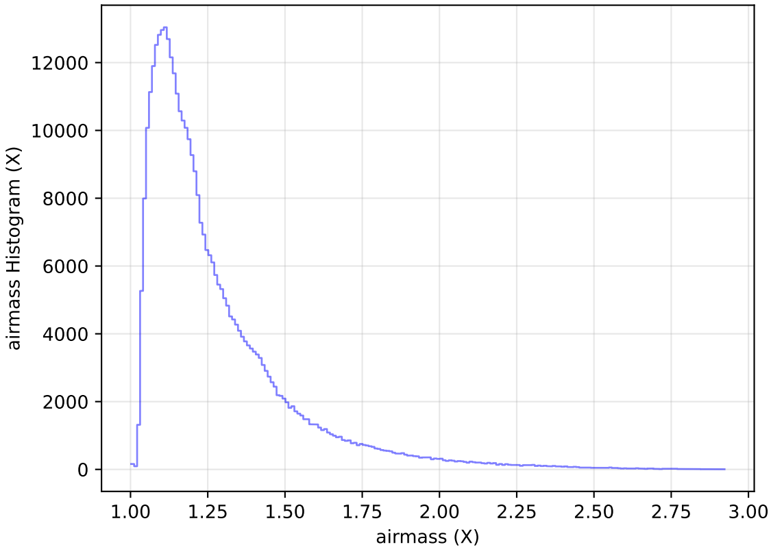
too_100_4v3.4_10yrs All sky y band: airmass Histogram
