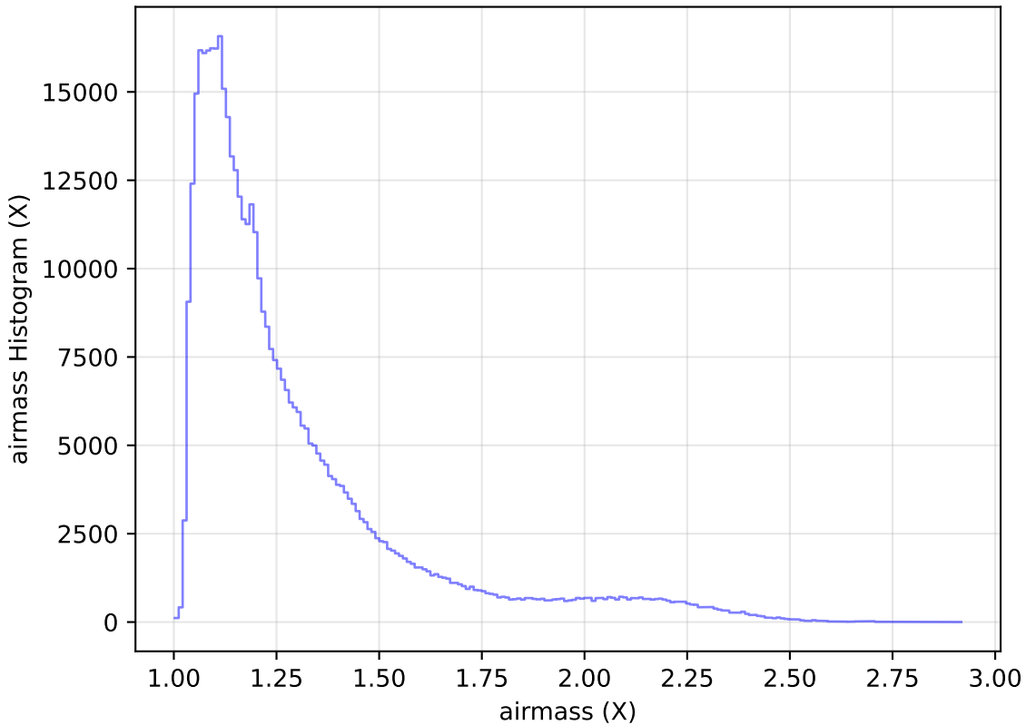
too_100_4v3.4_10yrs All sky r band: airmass Histogram
