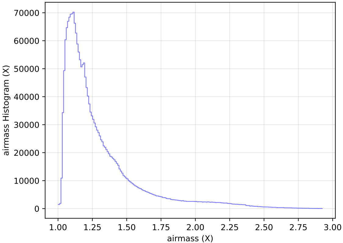
too_100_4v3.4_10yrs All sky all bands: airmass Histogram
