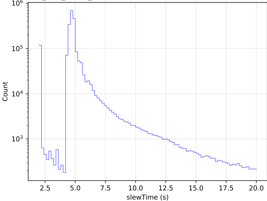
too_100_4v3.4_10yrs All visits: Zoom Slew Time Histogram
