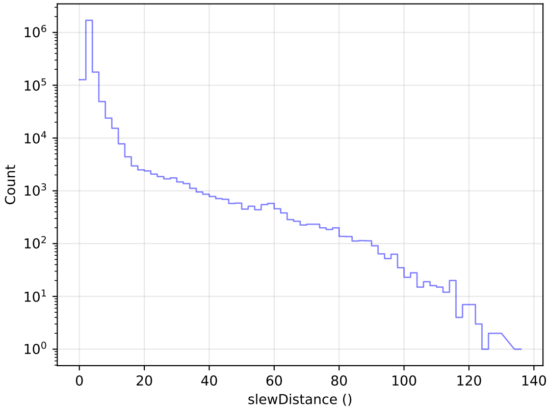
too_100_4v3.4_10yrs All visits: Slew Distance Histogram
