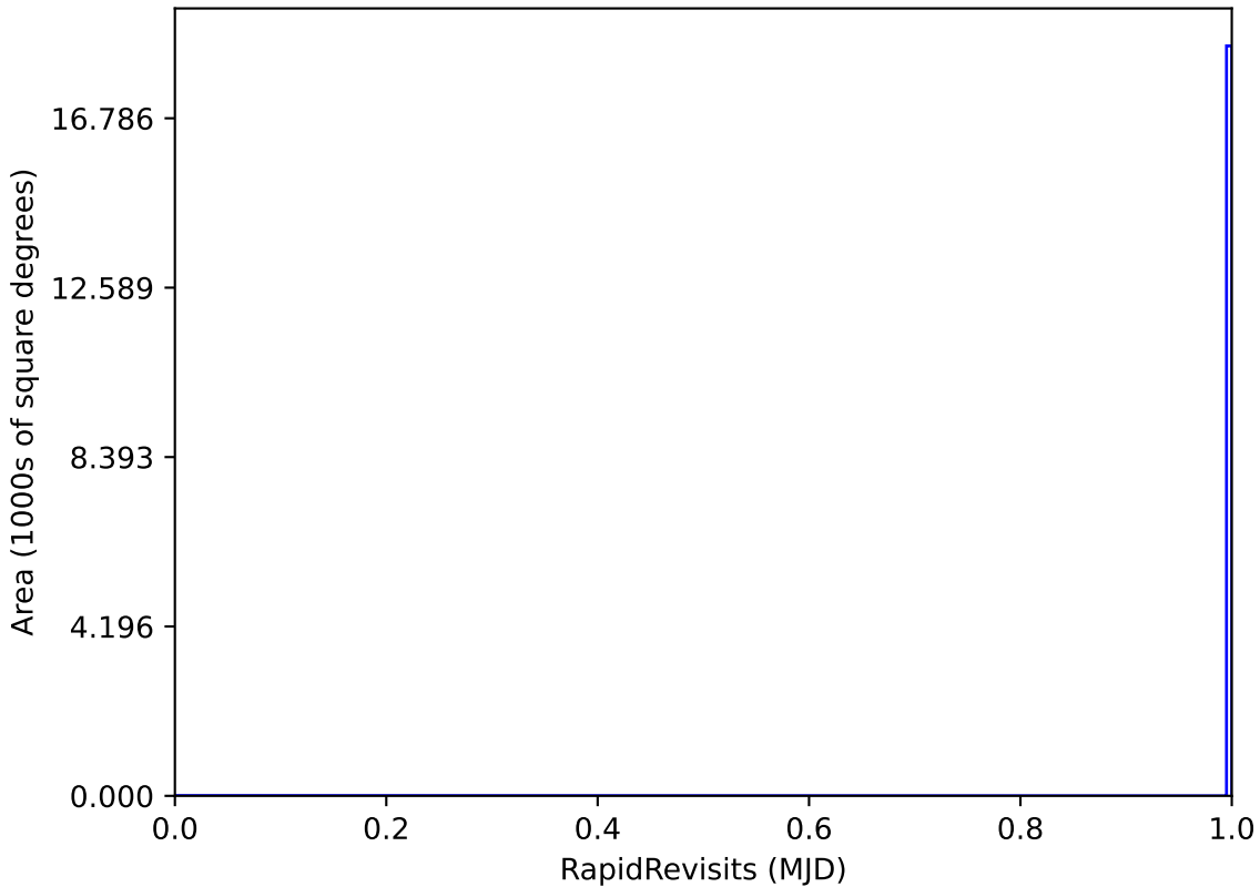
too_100_4v3.4_10yrs WFD: RapidRevisits
