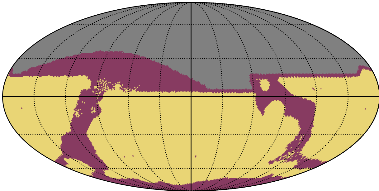
too_100_4v3.4_10yrs All sky: RapidRevisits
