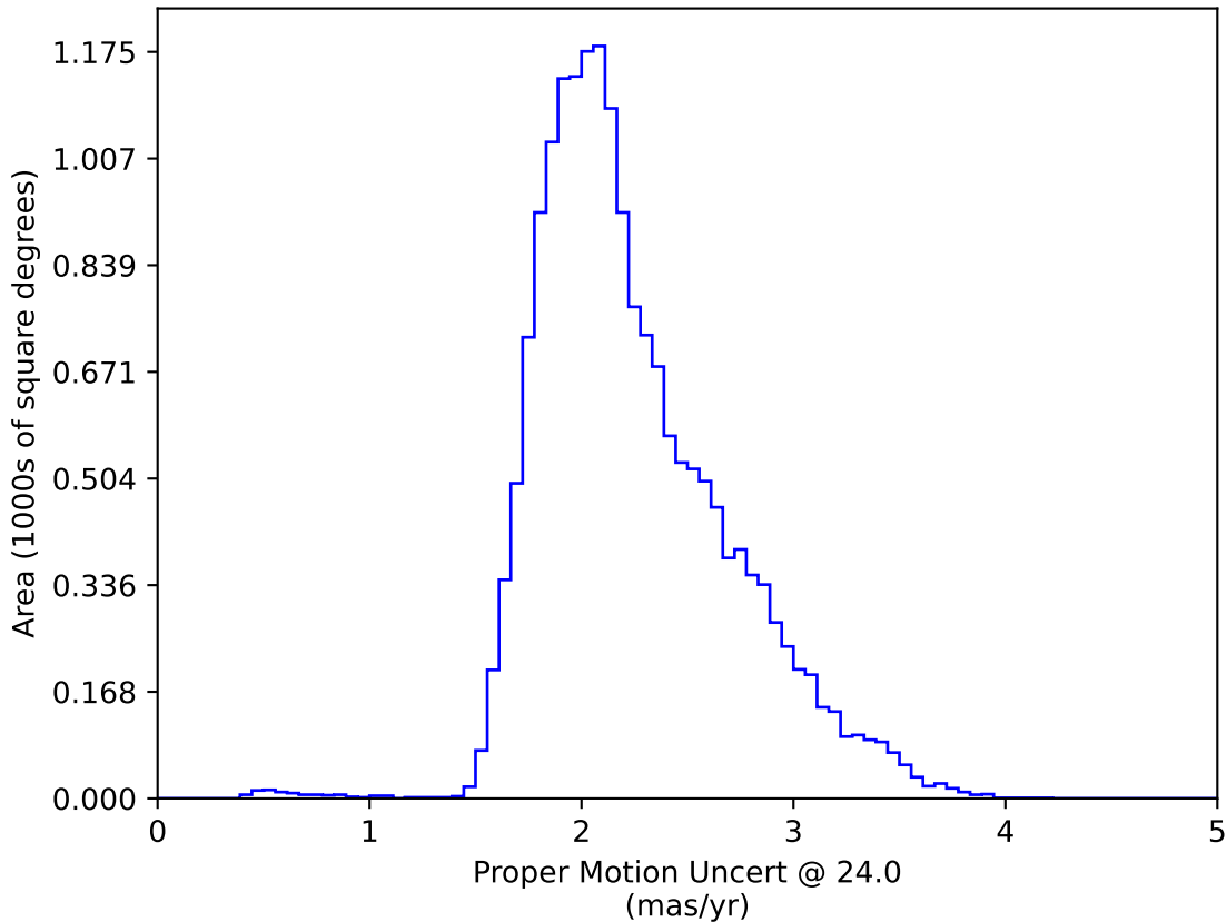
too_100_4v3.4_10yrs WFD: Proper Motion Uncert @ 24.0
