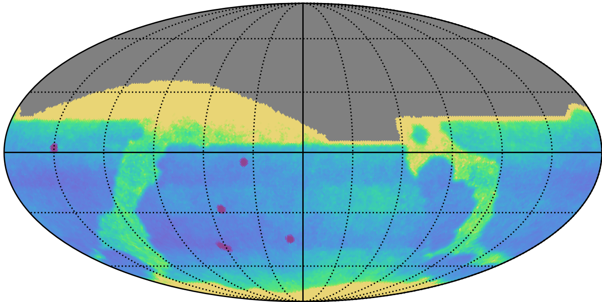
too_100_4v3.4_10yrs All sky: Proper Motion Uncert @ 24.0
