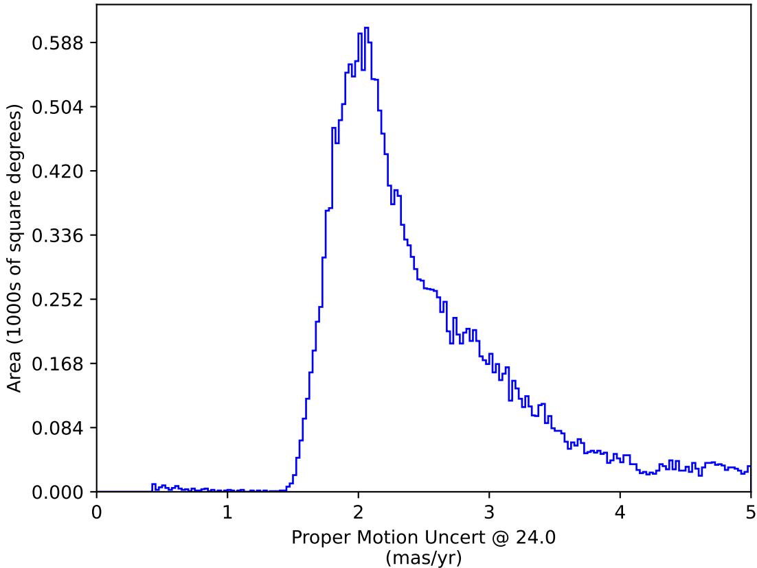
too_100_4v3.4_10yrs All sky: Proper Motion Uncert @ 24.0
