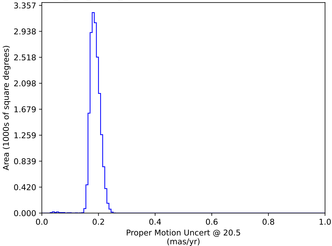
too_100_4v3.4_10yrs WFD: Proper Motion Uncert @ 20.5
