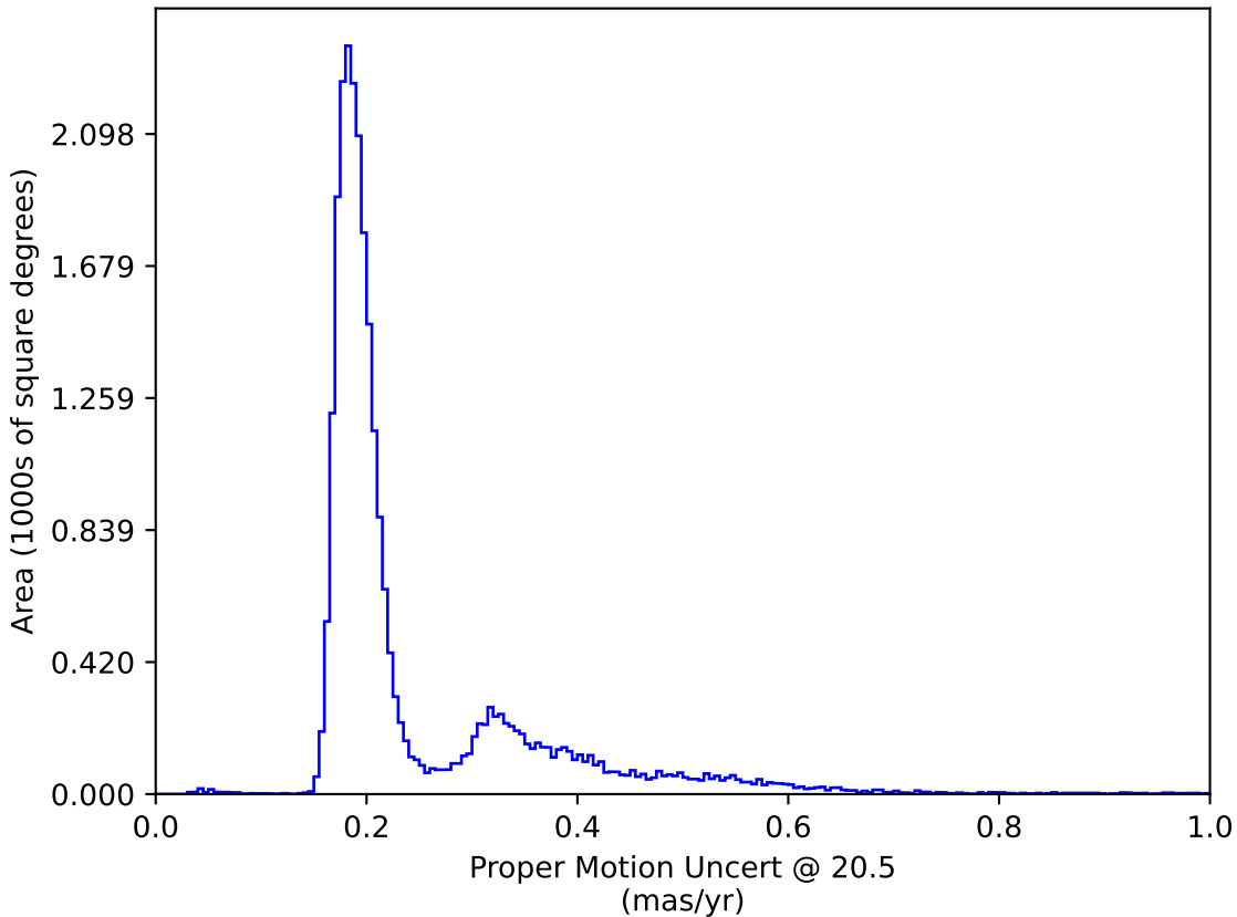
too_100_4v3.4_10yrs All sky: Proper Motion Uncert @ 20.5
