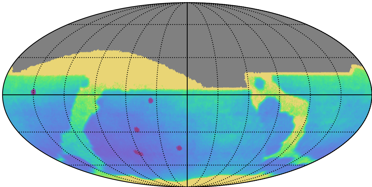
too_100_4v3.4_10yrs All sky: Parallax Uncert @ 22.4
