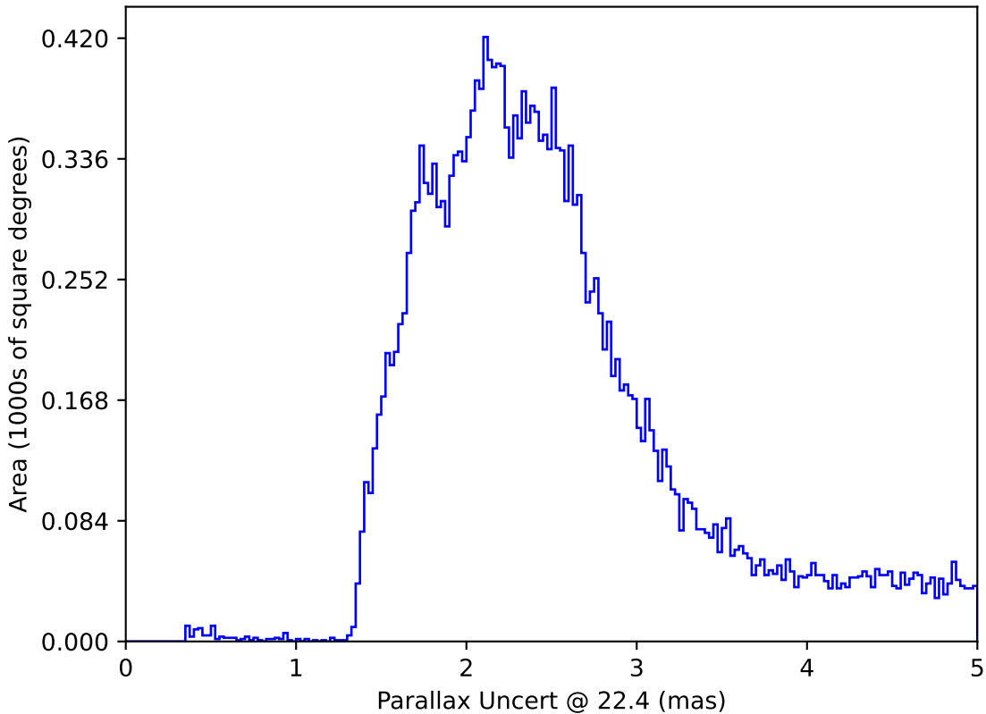
too_100_4v3.4_10yrs All sky: Parallax Uncert @ 22.4
