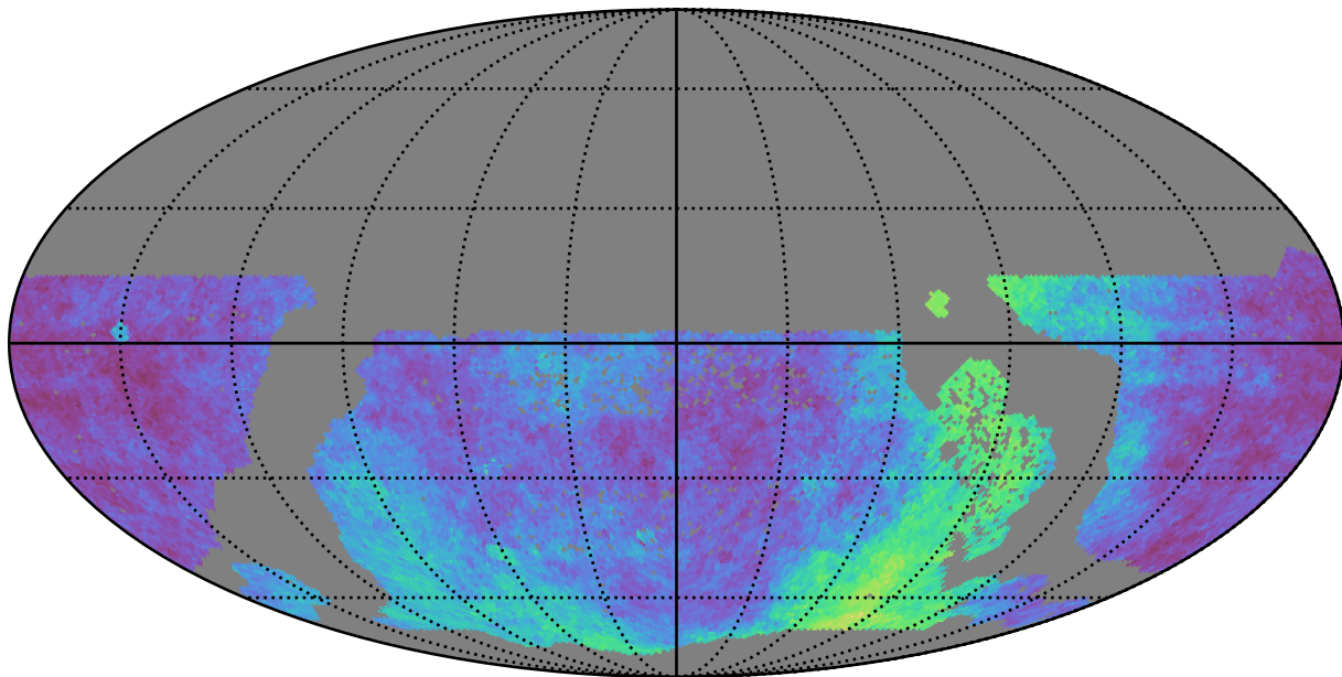
too_100_4v3.4_10yrs WFD: Parallax Coverage @ 24.0
