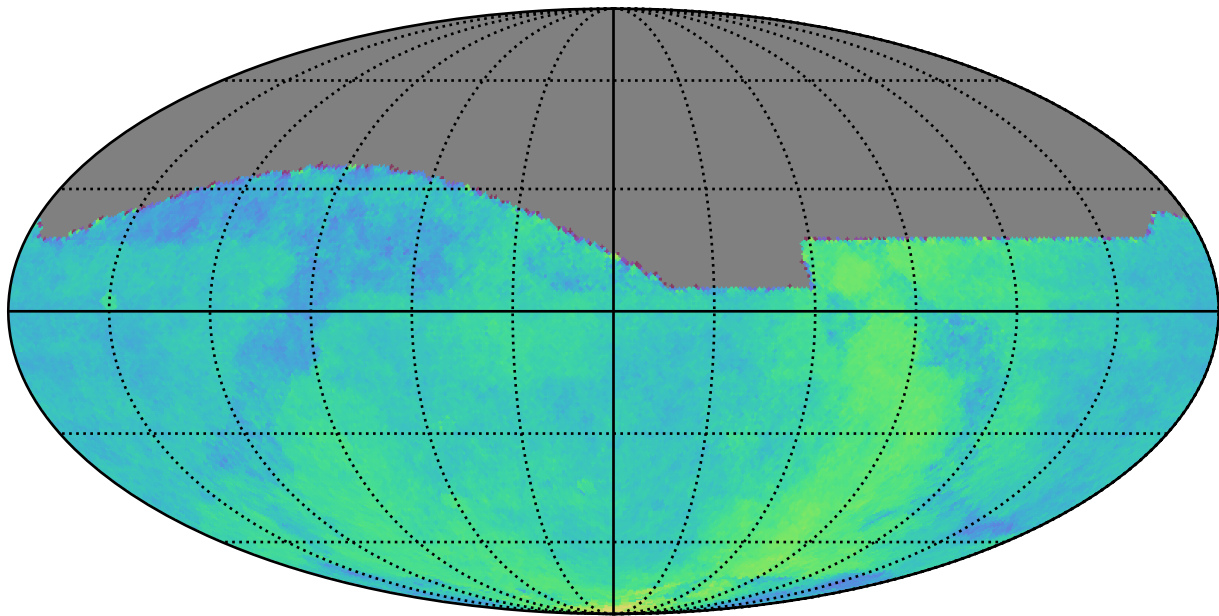
too_100_4v3.4_10yrs All sky: Parallax Coverage @ 24.0
