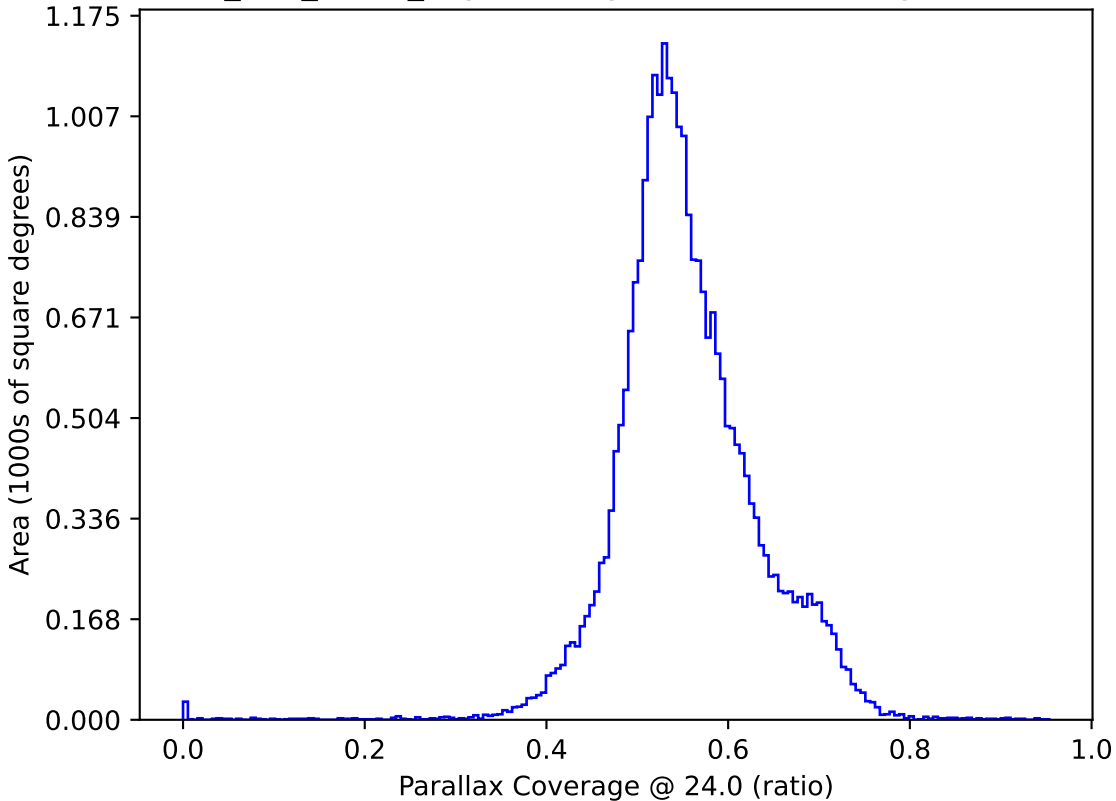
too_100_4v3.4_10yrs All sky: Parallax Coverage @ 24.0
