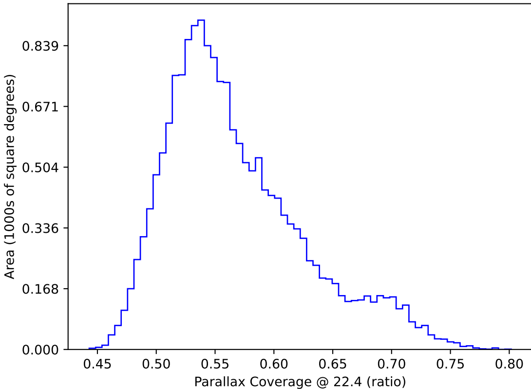
too_100_4v3.4_10yrs WFD: Parallax Coverage @ 22.4
