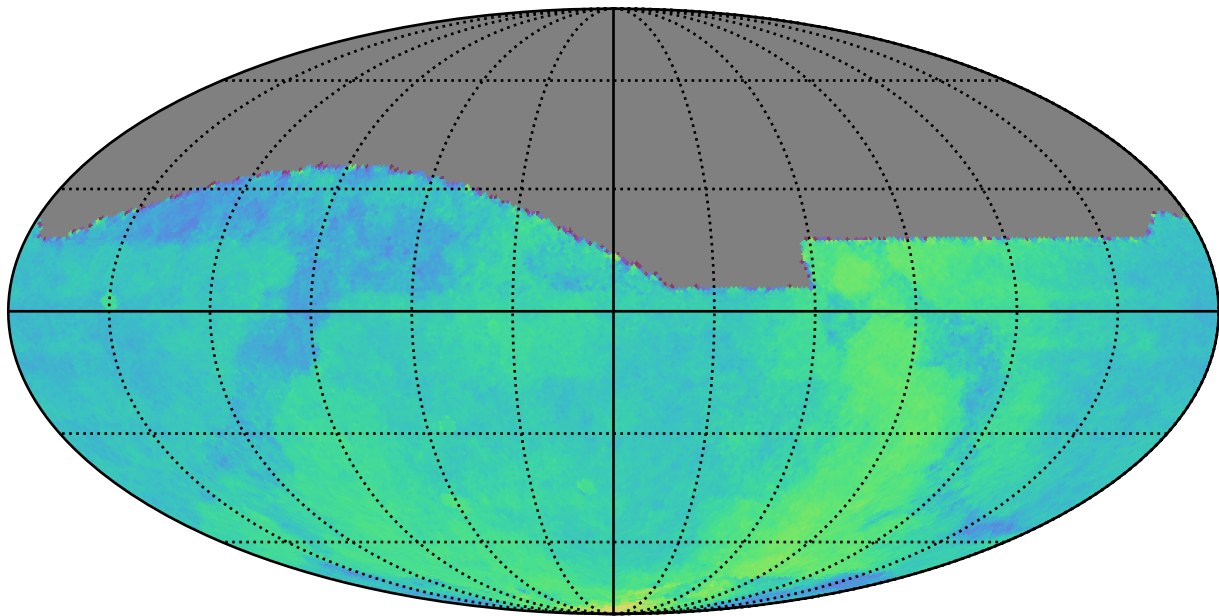
too_100_4v3.4_10yrs All sky: Parallax Coverage @ 22.4
