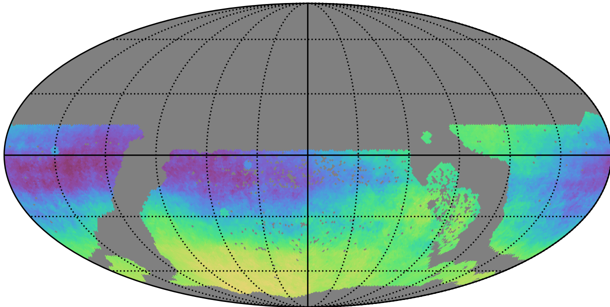
too_100_4v3.4_10yrs WFD: Parallax-DCR degeneracy @ 24.0
