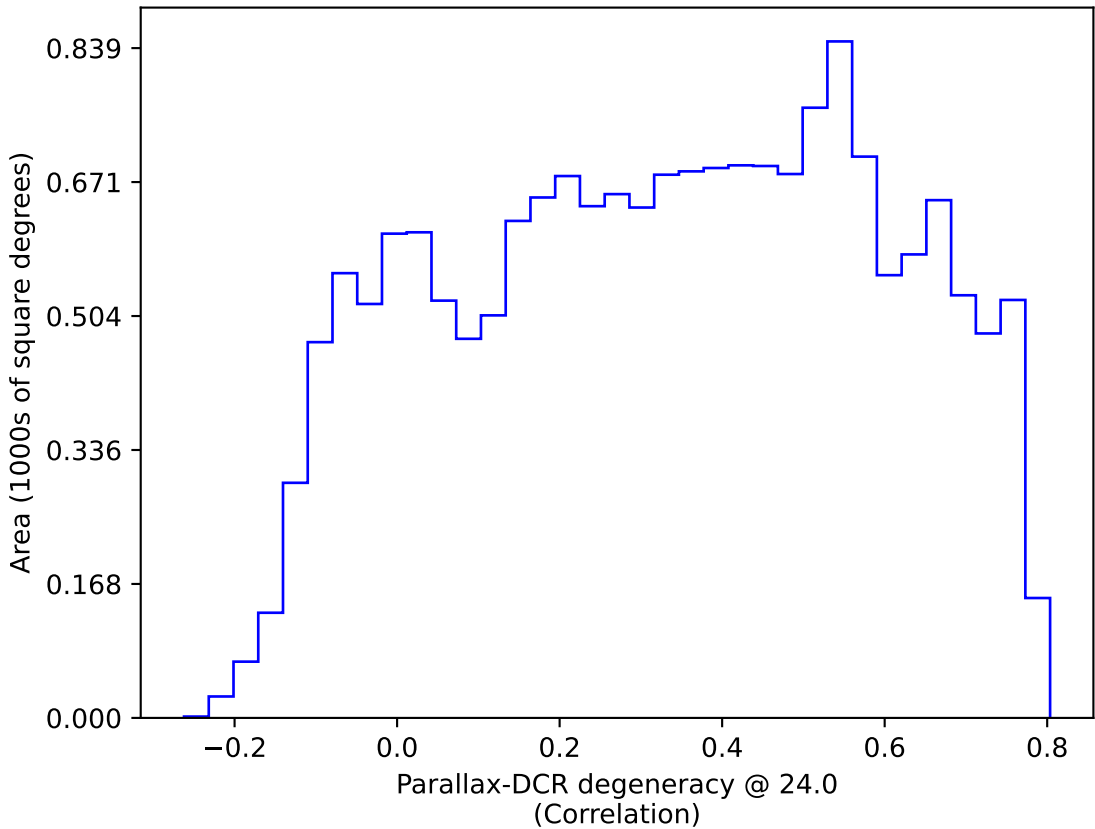
too_100_4v3.4_10yrs WFD: Parallax-DCR degeneracy @ 24.0
