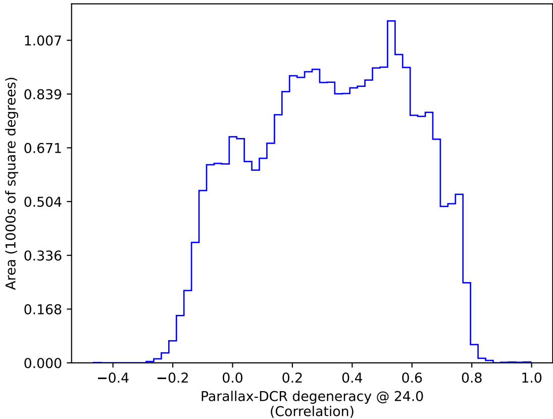
too_100_4v3.4_10yrs All sky: Parallax-DCR degeneracy @ 24.0
